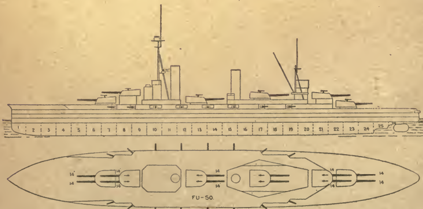
JAPANESE DREADNOUGHT FU-50
